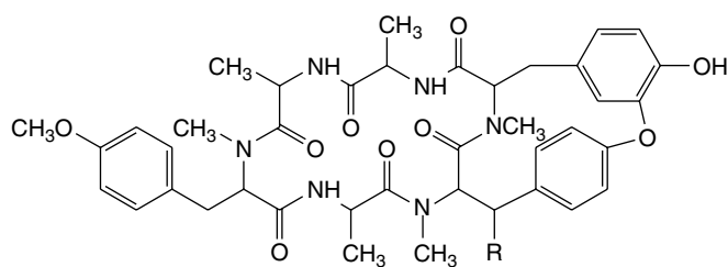
Bouvardin, R = OH
