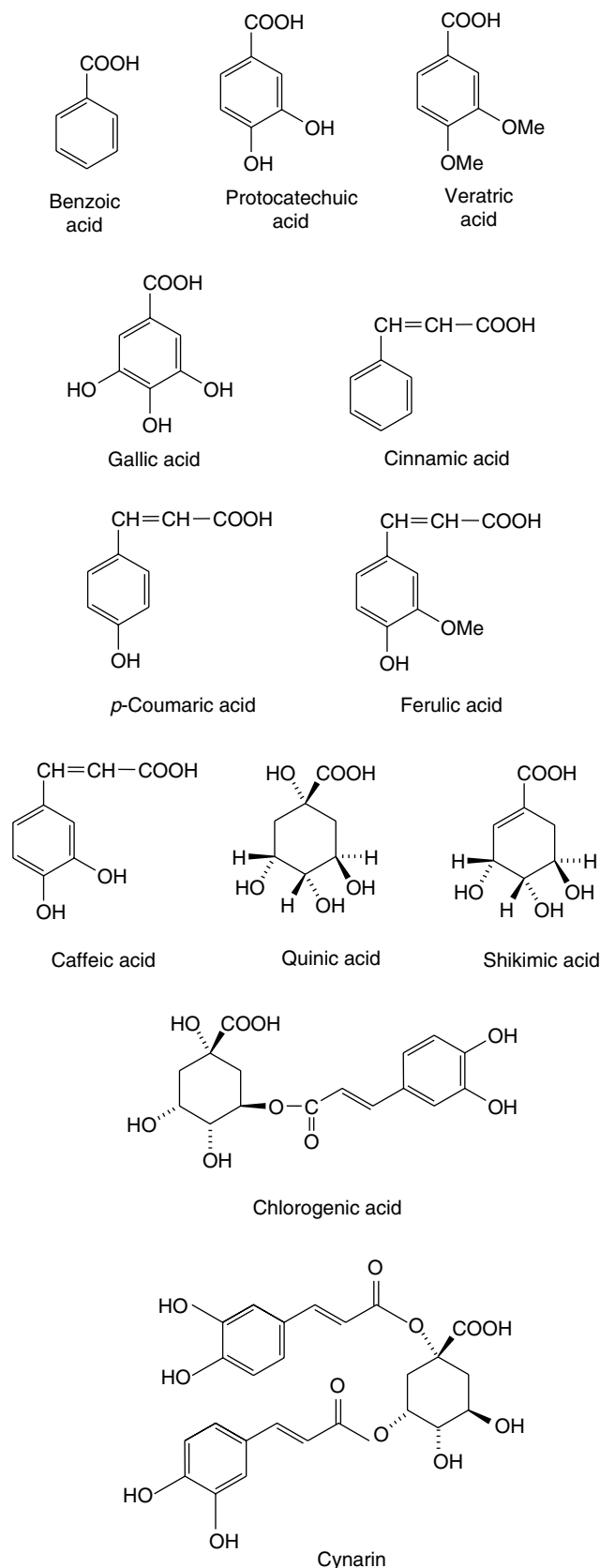
Fig. 19.5 Aromatic and other cyclic acids.
