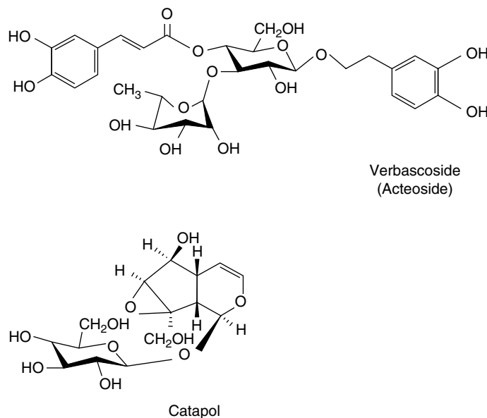
Fig. 20.7 Constituents of mullein flowers.
