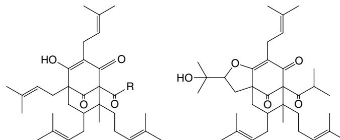
Hyperforin, R = CH(CH 3 ) 2 Adhyperforin, R = CH(CH 3 )CH 2 CH 3
