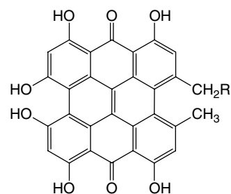
Hypericin, R = H Pseudohypericin, R = OH
