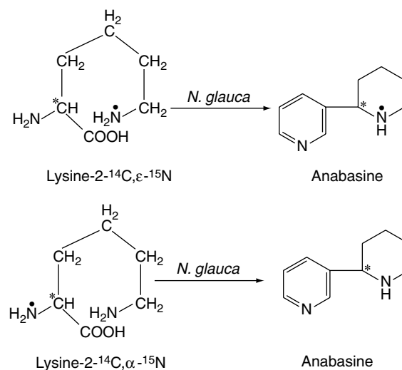
Fig. 17.4 Incorporation of doubly-labelled lysines into anabesine.
