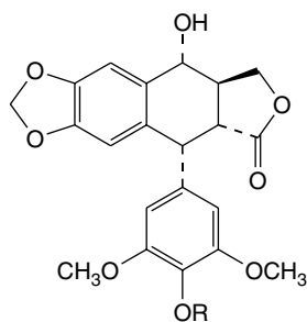
Podophyllotoxin, R = CH 3
