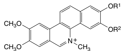
Fagaronine, R 1 = H, R 2 = CH 3
