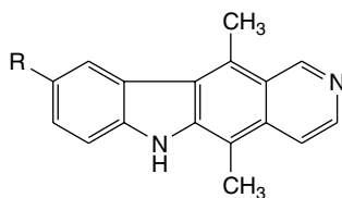
Ellipticine, R = H
