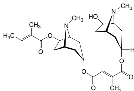
Schizanthine Z—a tropanol diol mesaconic acid diester
