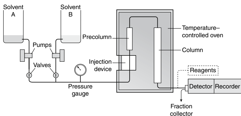
Fig. 17.1 Schematic representation of apparatus for high-performance liquid chromatography utilizing two solvents.
